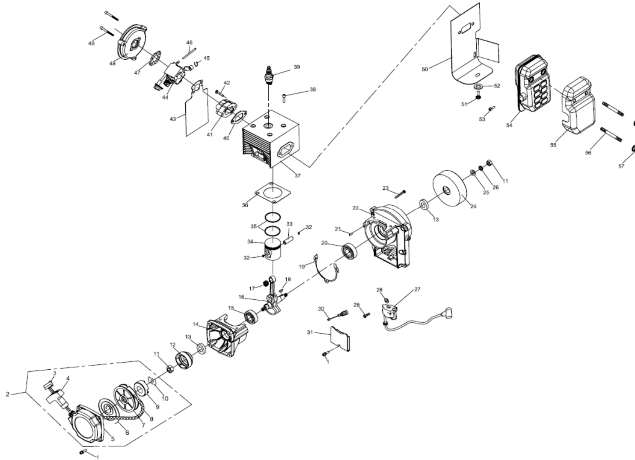
Fig. 1 ENGINE GROUP
